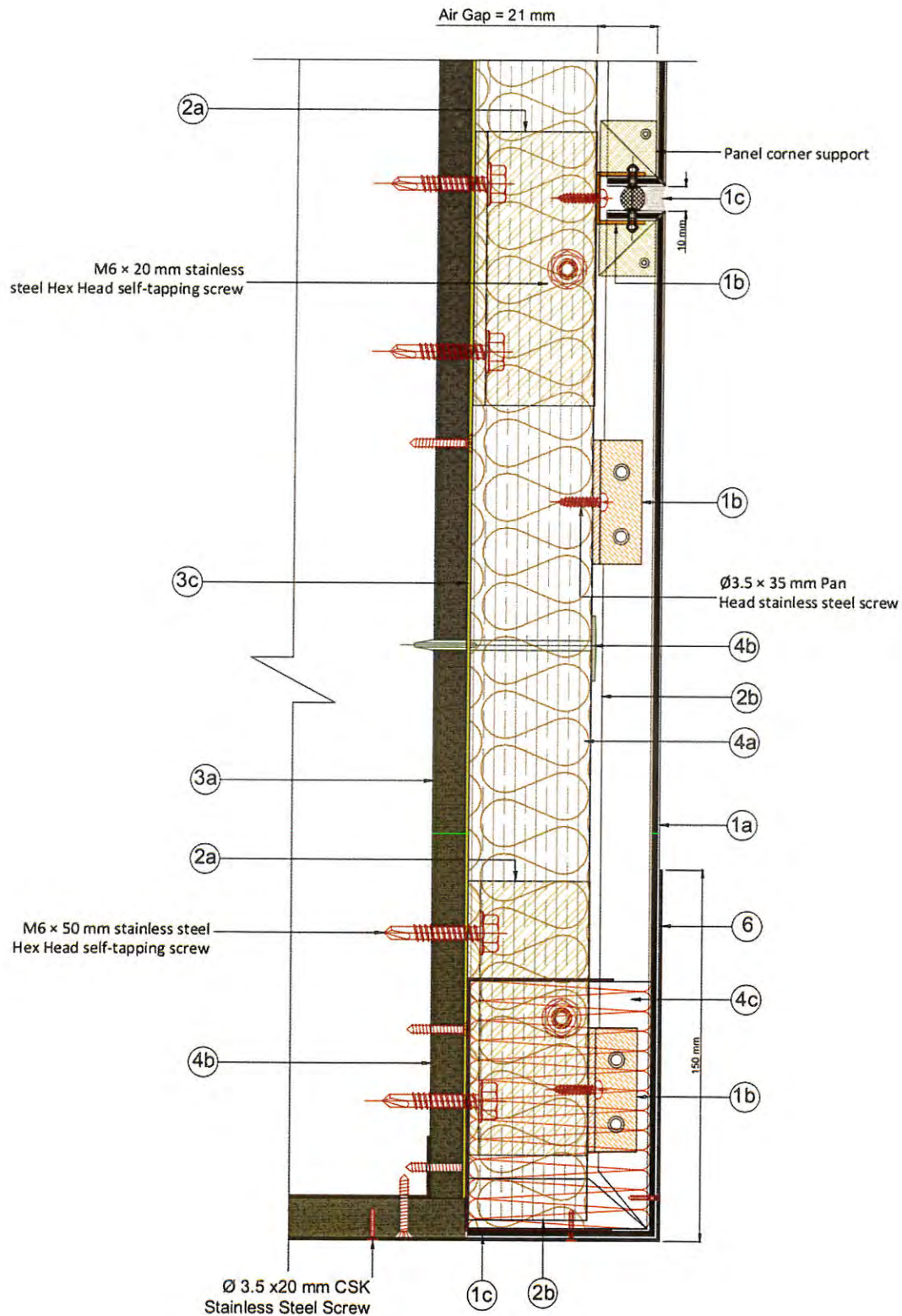
Figure 2. "Alucopanel® A2" 4 mm thick Aluminium Composite Material "Close-Joint" Non-Loadbearing Exterior Wall Cladding Assembly vertical window section details
