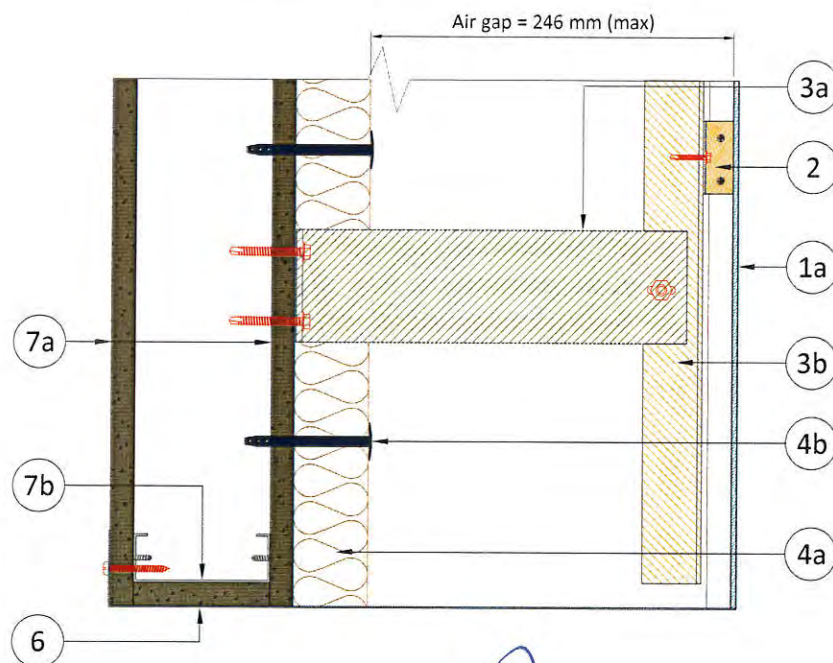
Figure 5. Vertical section – window details
