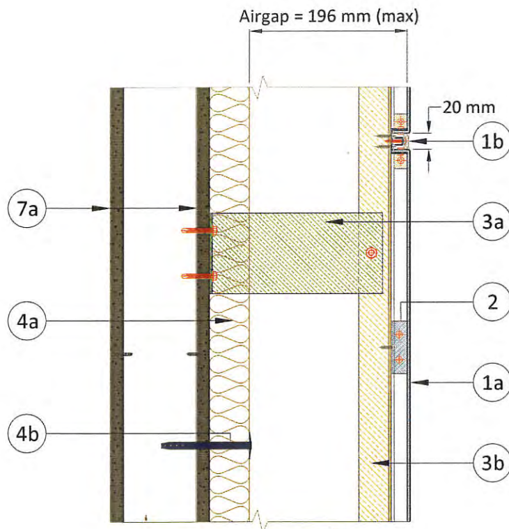
Figure 3. Vertical section – joint details
