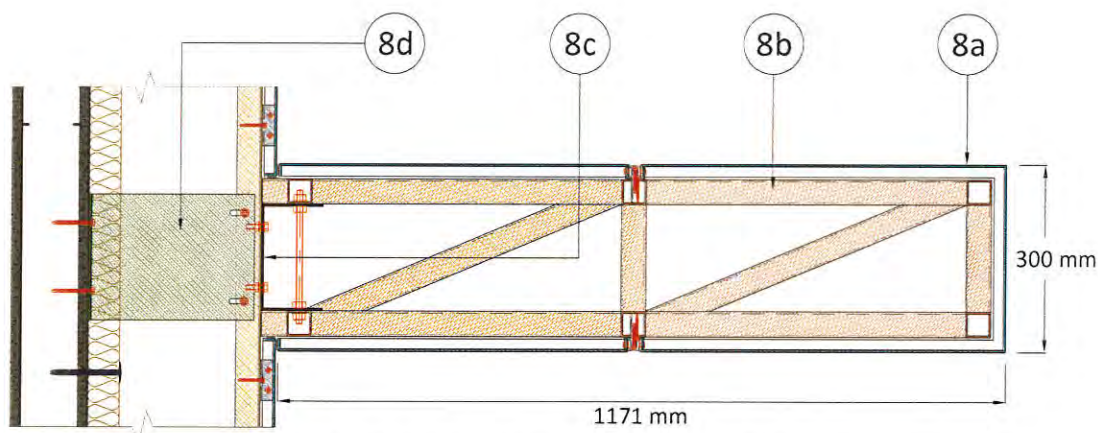
Figure 6. Vertical Section – Canopy and Soffit Details
