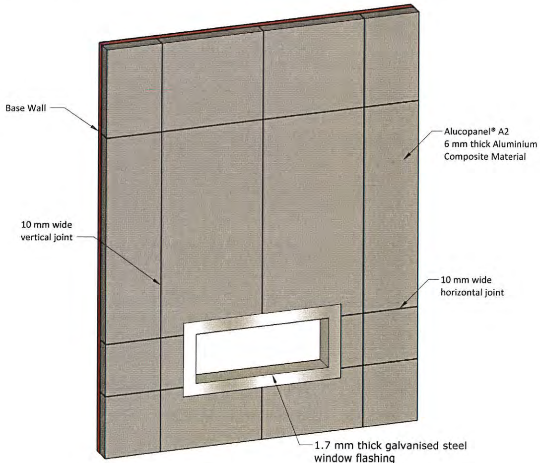
Figure 1. Aluminium Composite Material Exterior Wall Cladding System
