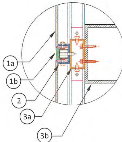
Figure 3b. Detail A
