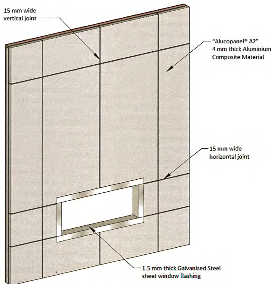
Figure 1. Aluminium Composite Material Non-Loadbearing Exterior Wall Cladding System
