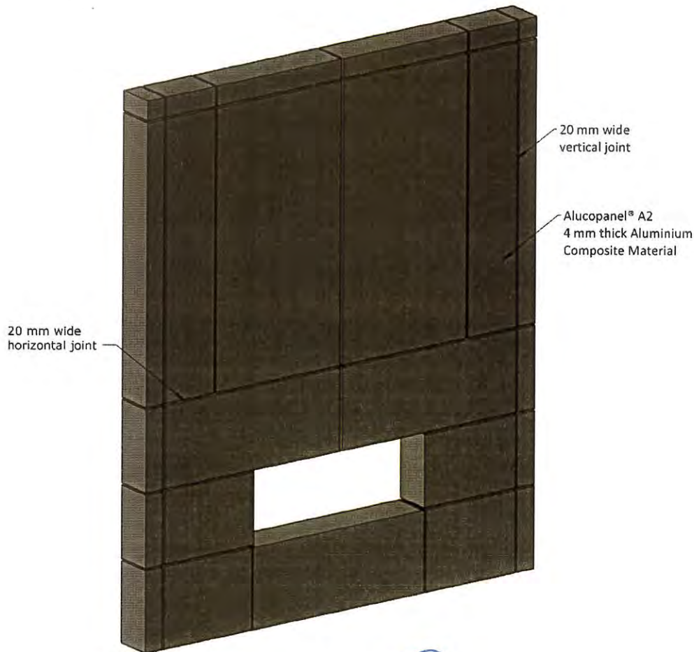
Figure 1. Aluminium Composite Material Exterior Wall Cladding System
