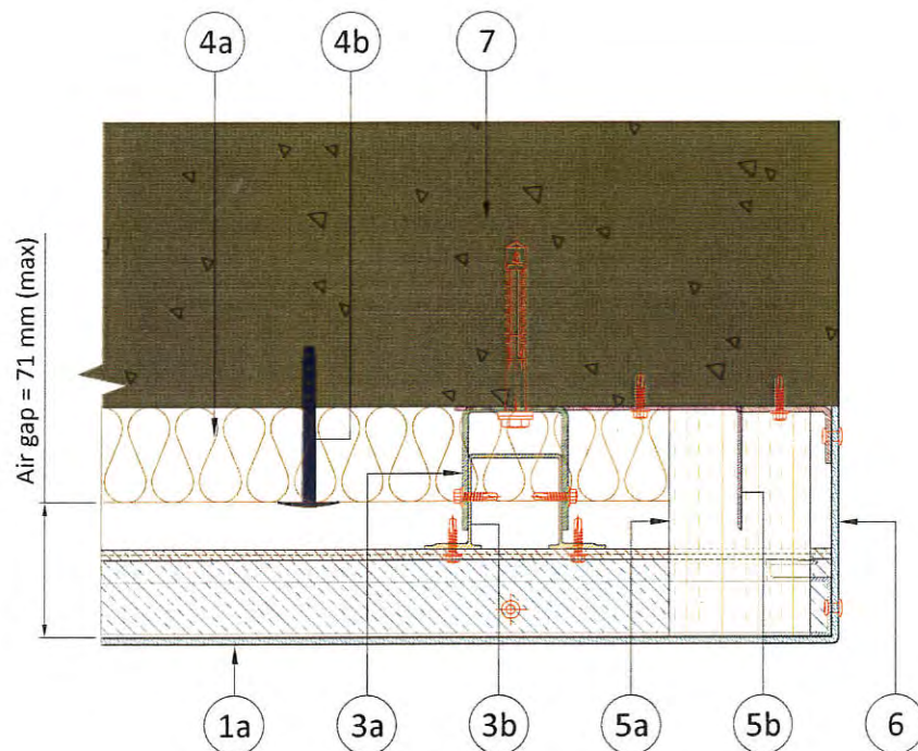
Figure 4. Horizontal section – window details
