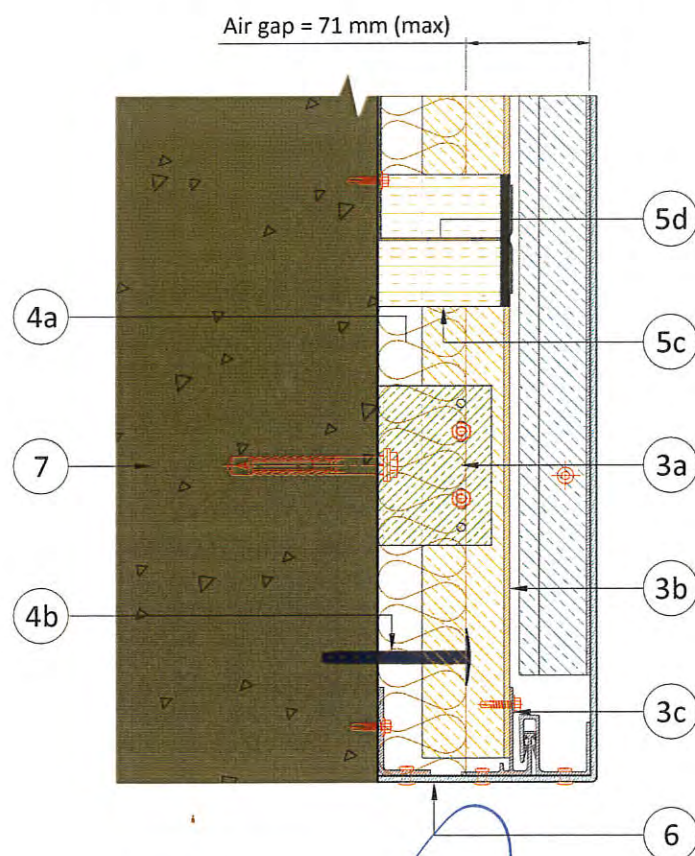
Figure 5. Vertical section – window details
