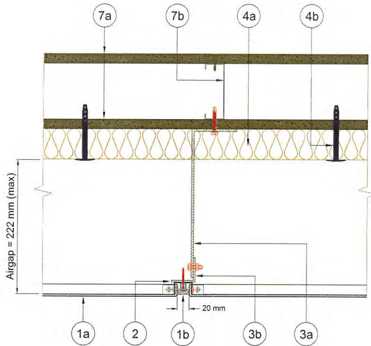
Figure 2. Horizontal section – joint details
