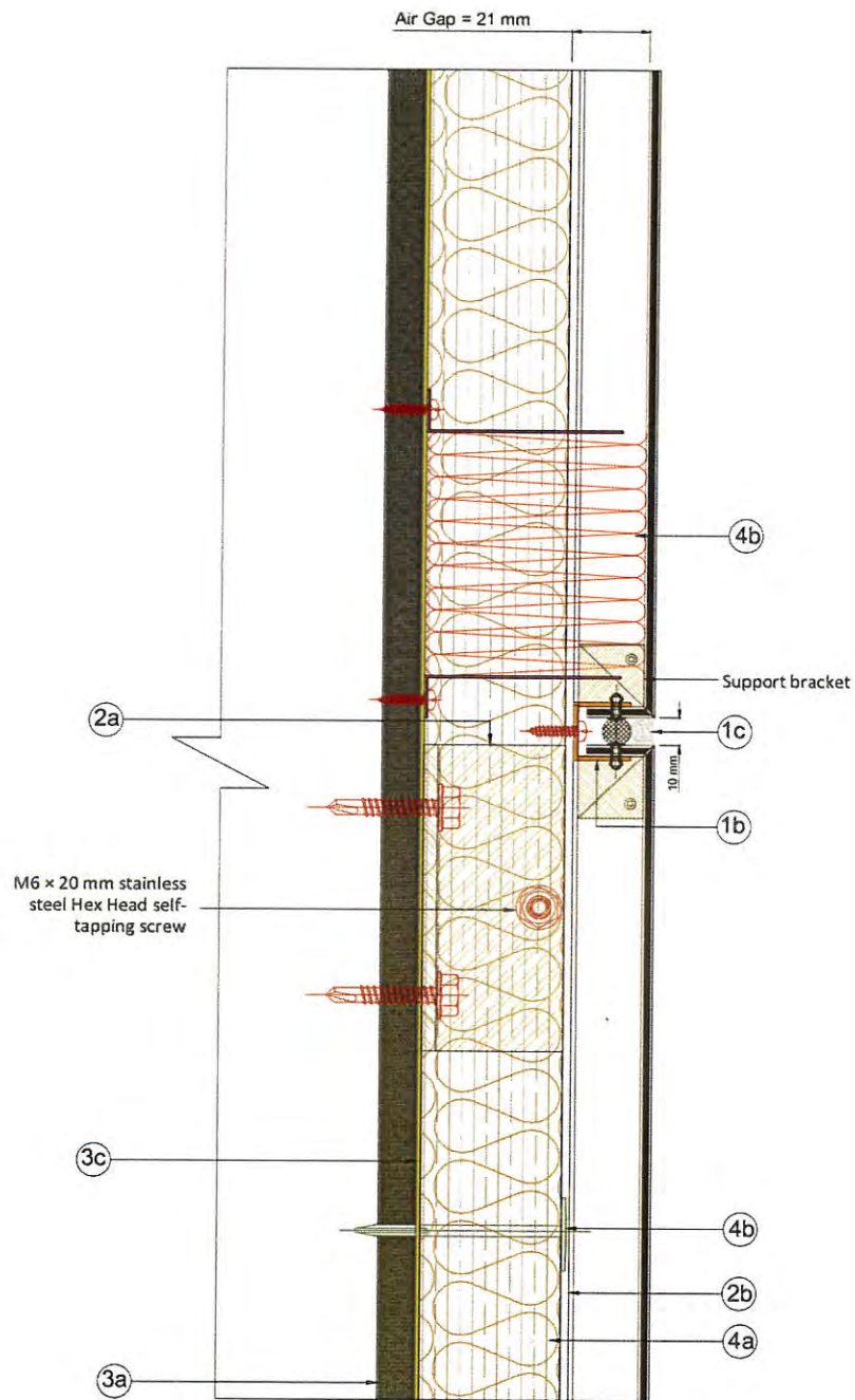
Figure 3. "Alucopanel® A2" 4 mm thick Aluminium Composite Material "Close-Joint" Non-Loadbearing Exterior Wall Cladding Assembly vertical section details
