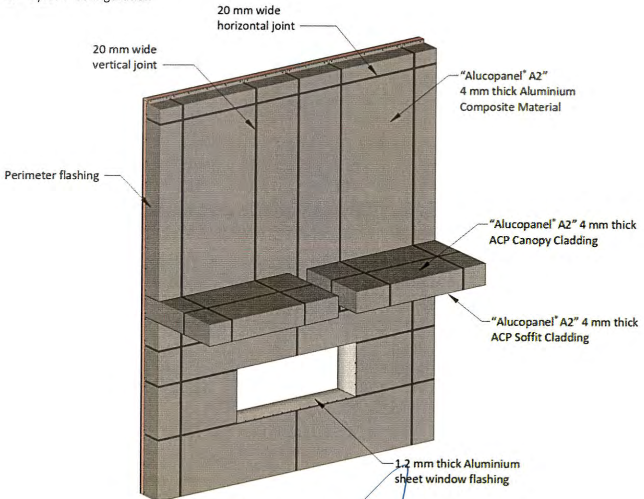
Figure 1. Aluminium Composite Material Exterior Wall Cladding System
