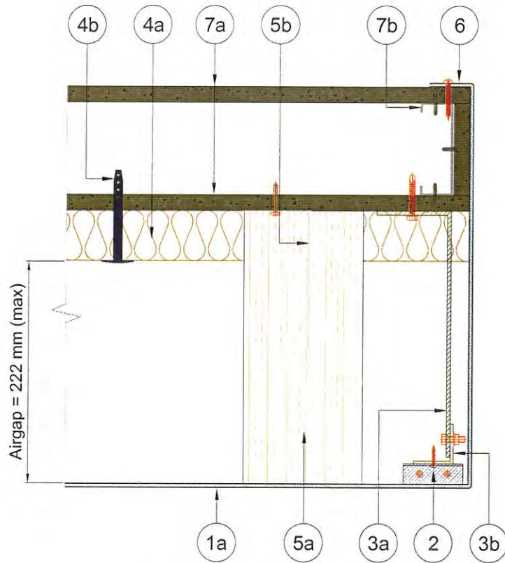
Figure 4. Horizontal section – window details
