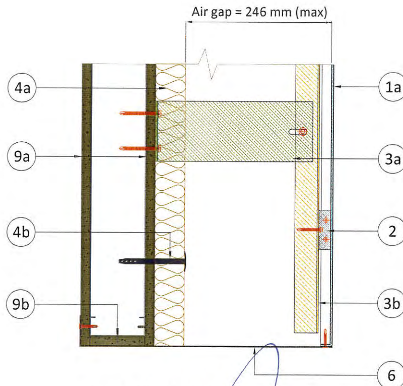
Figure 5. Vertical Section – Window Details
