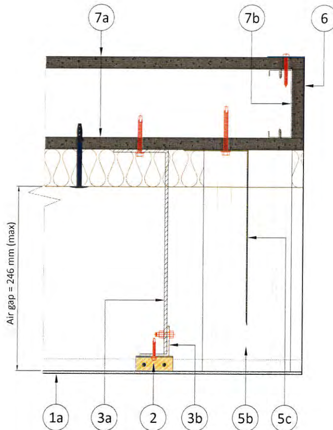
Figure 4. Horizontal section – window details
