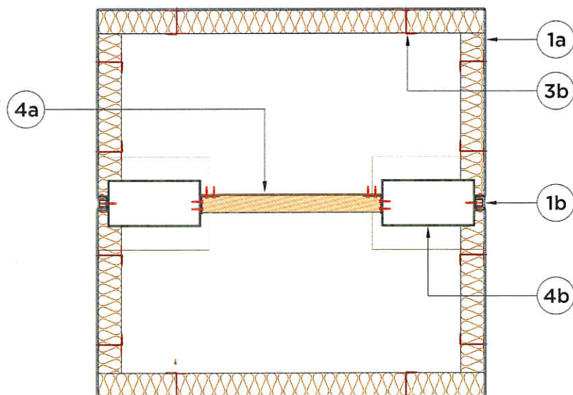
Figure 2. Section A-A
