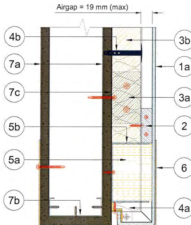
Figure 5. Vertical section – window details
