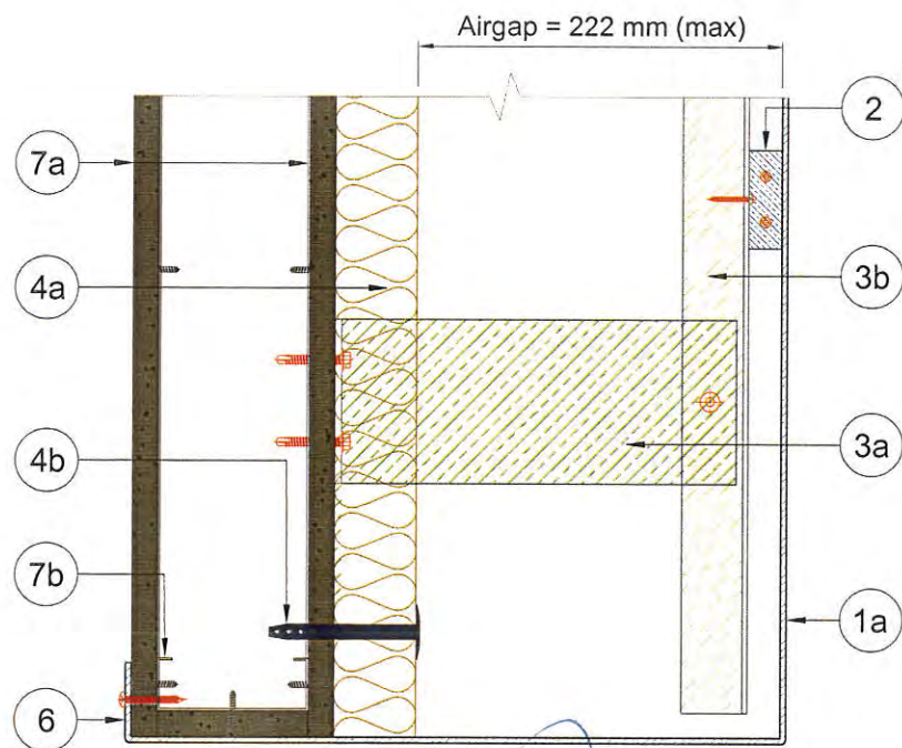
Figure 5. Vertical section – window details
