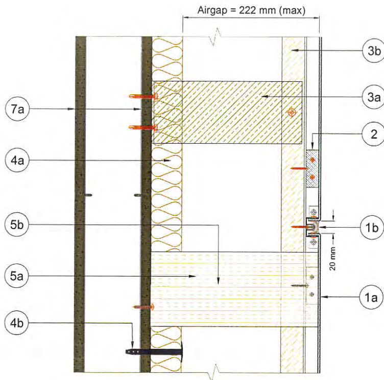
Figure 3. Vertical section – joint details
