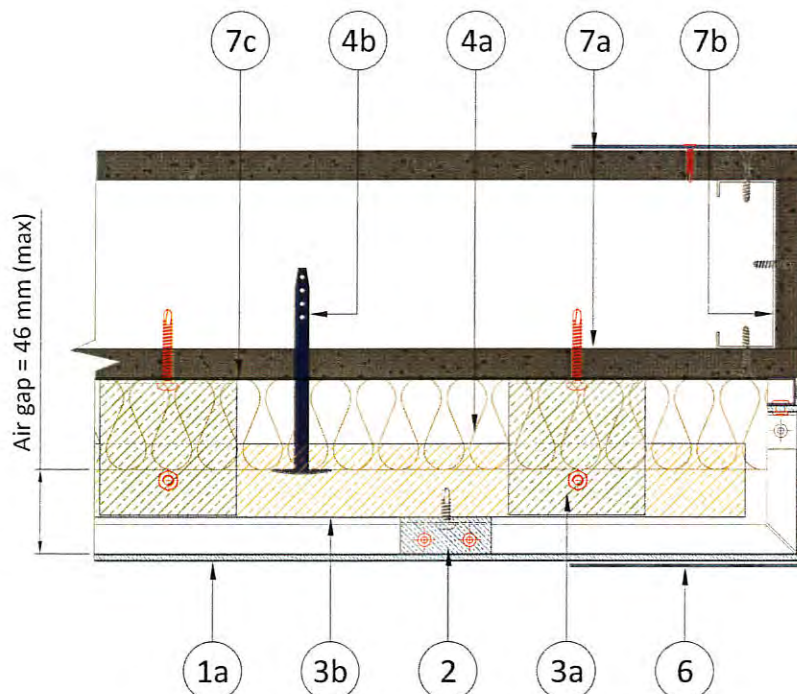
Figure 4. Horizontal Section – Window Details
