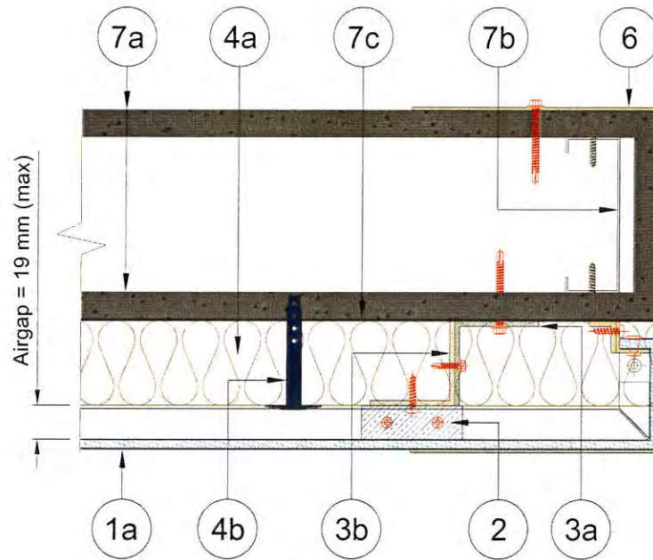
Figure 4. Horizontal section – window details
