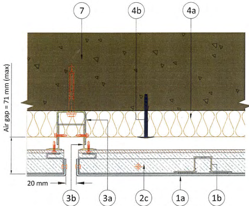
Figure 2. Horizontal section – joint details
