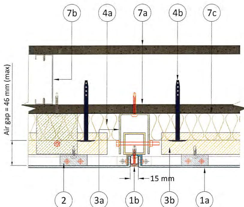
Figure 2. Horizontal Section – Joint Details
