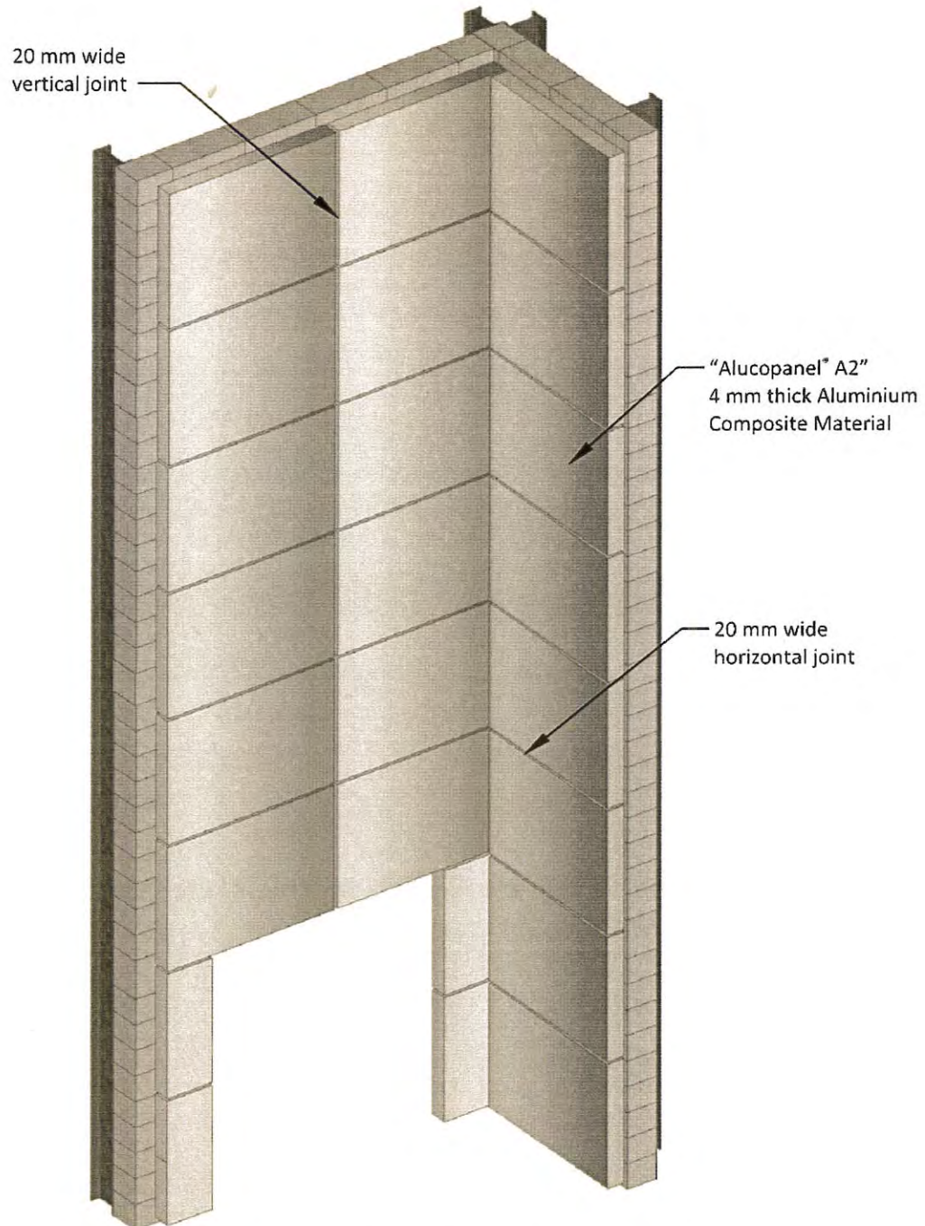
Figure 1. Aluminium Composite Material Exterior Wall Cladding System
