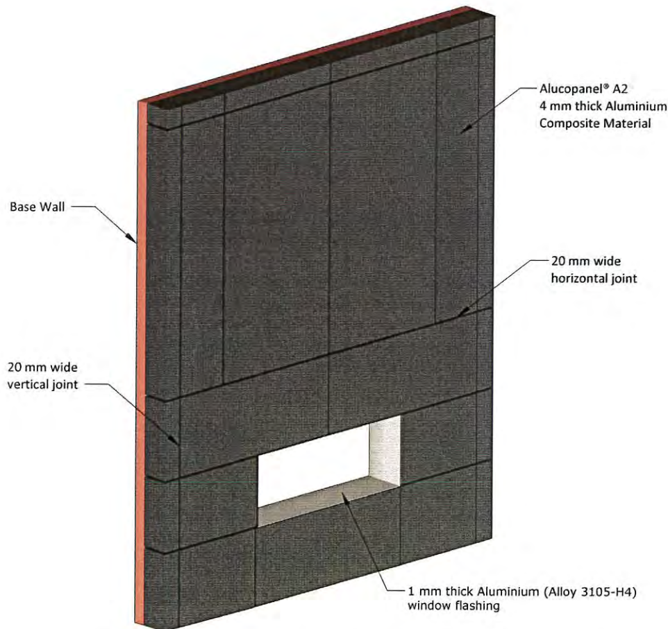
Figure 1. Aluminium Composite Material Exterior Wall Cladding Assembly
