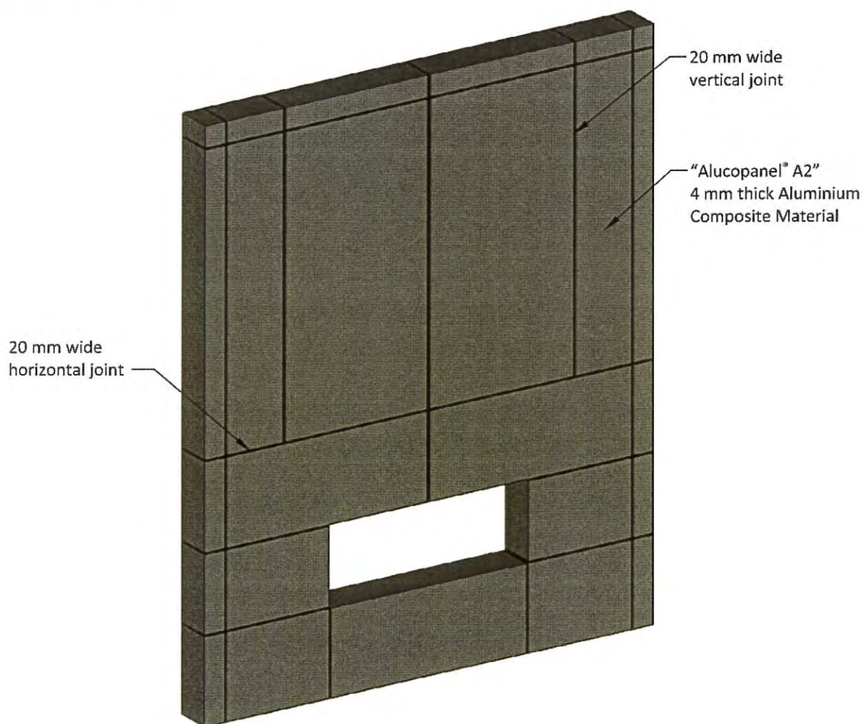
Figure 1. Aluminium Composite Material Exterior Wall Cladding System
