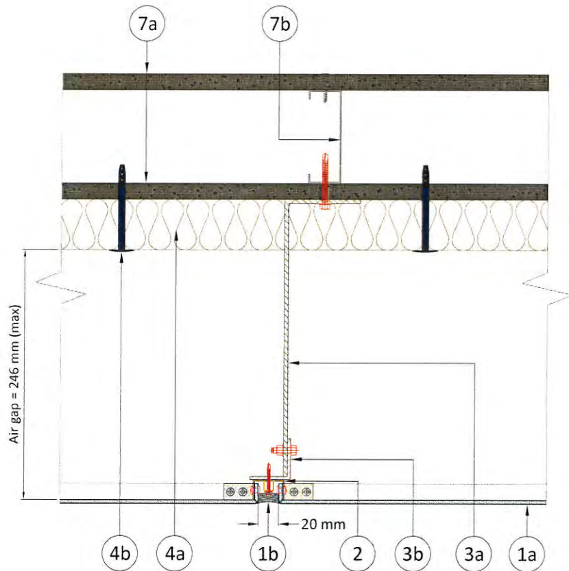
Figure 2. Horizontal section – joint details
