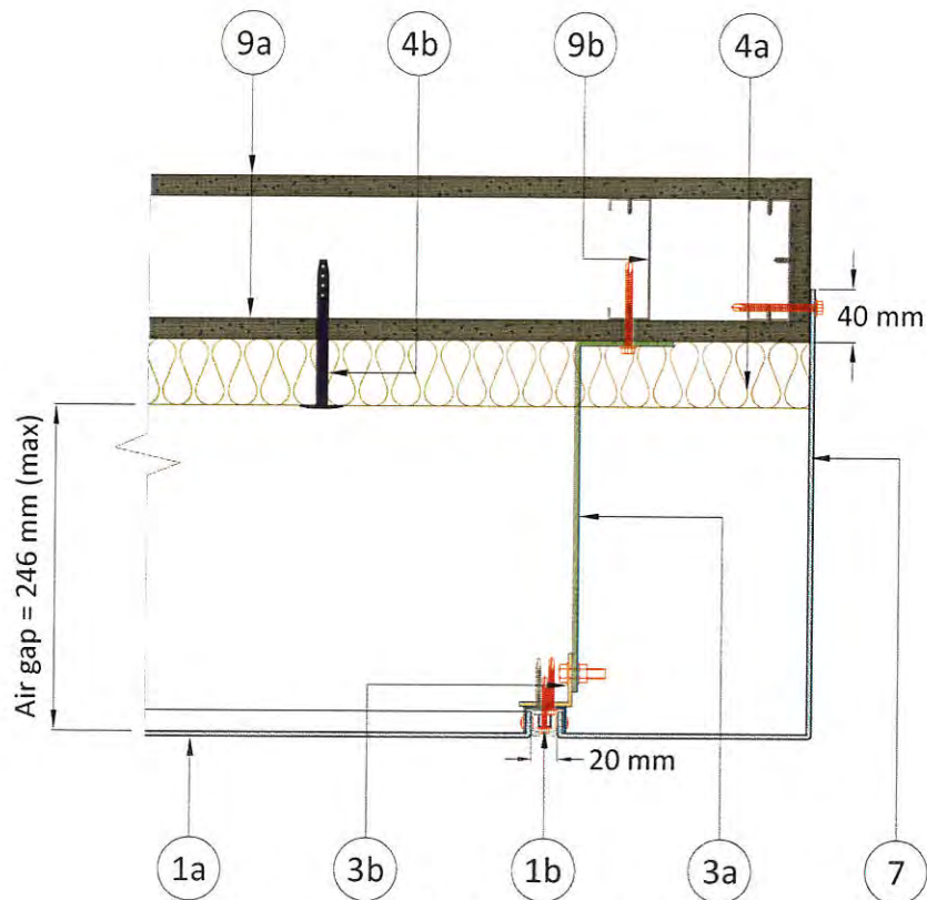
Figure 2. Horizontal Section – Joint Details
