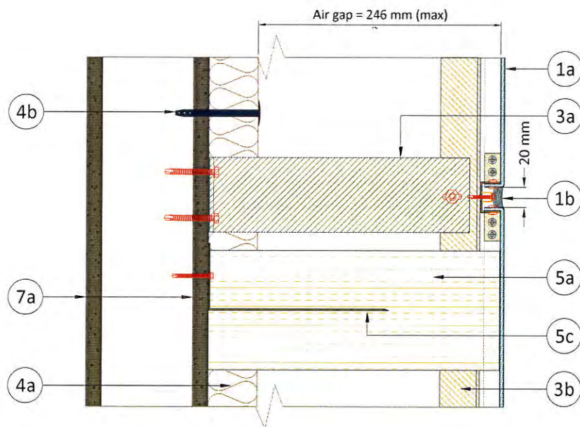
Figure 3. Vertical section – joint details
