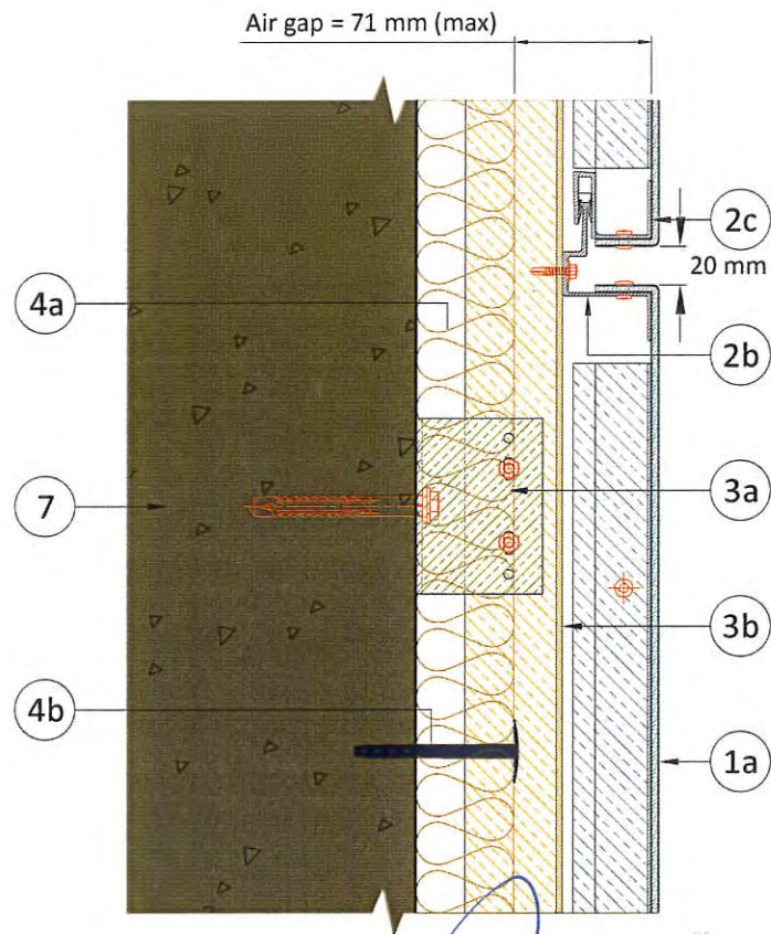
Figure 3. Vertical section – joint details
