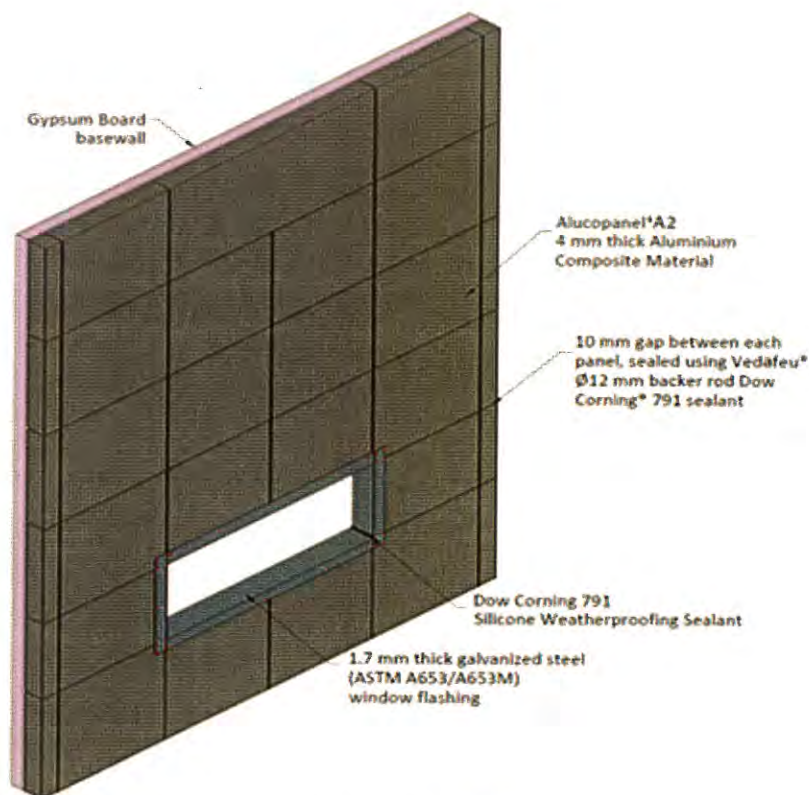
Figure 1. "Alucopanel® A2" 4 mm thick Aluminium Composite Material "Close-Joint" Non-Loadbearing Exterior Wall Cladding Assembly
