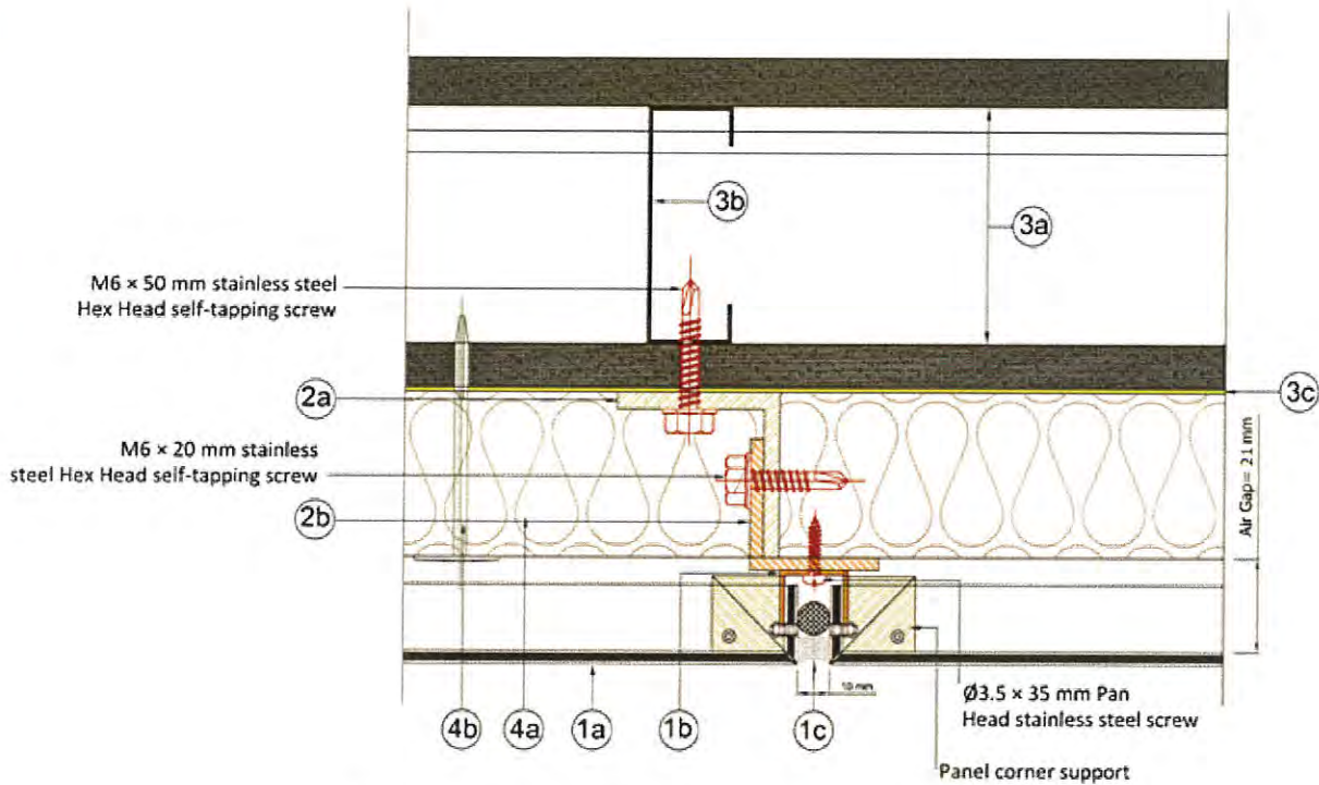
Figure 4. "Alucopanel® A2" 4 mm thick Aluminium Composite Material "Close-Joint" Non-Loadbearing Exterior Wall Cladding Assembly horizontal section details
