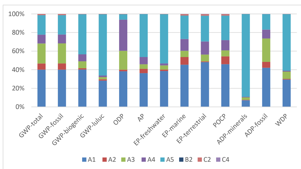
Figure 3. Contribution analysis for the Alucopanel® A1 products.
