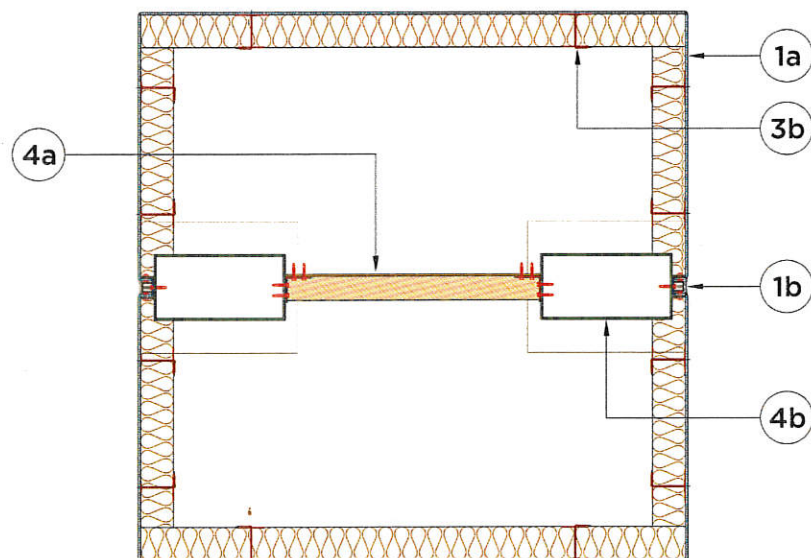
Figure 2. Section A-A
