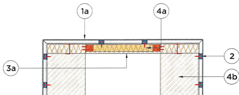
Figure 3. Section B-B
