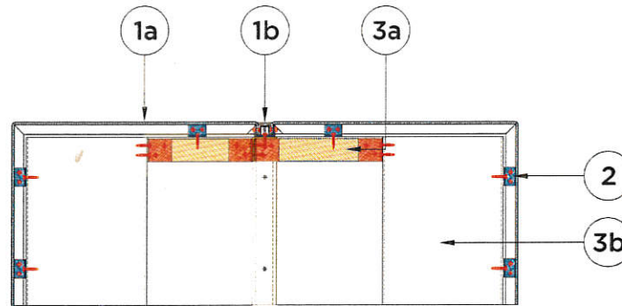
Figure 3. Section B-B
