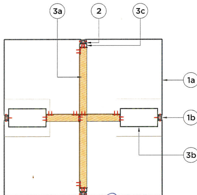
Figure 2. Section A-A
